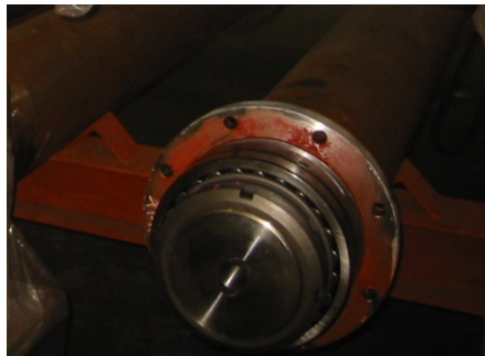
HLB (HARDLOCK Bearing Nut) M140 SS400
