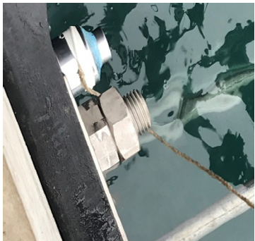
Fender HLN M56 SUS304
